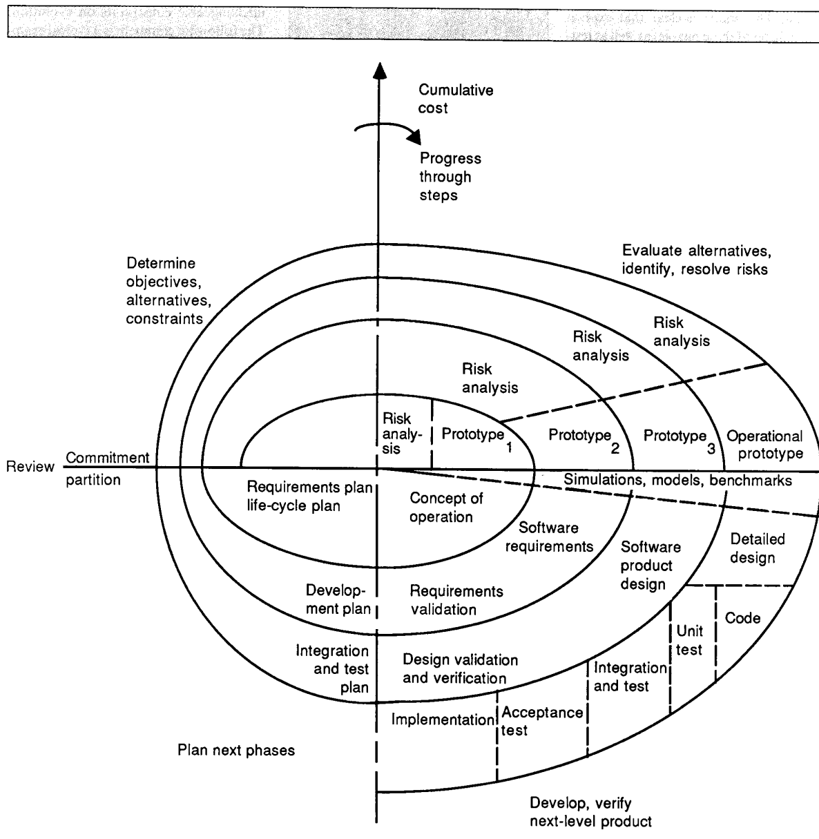
Figure 2. Spiral model of the software process.
